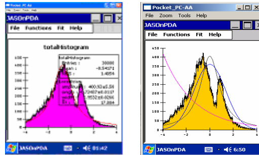
Figure 2. JASOnPDA running on a PDA showing its features of histogram plotting, function fitting, and statistics calculation.
