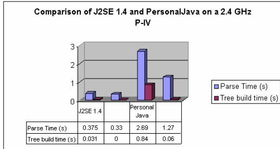
Figure 7. This chart shows that the performance disparity between Personal Java and J2SE 1.4 persists even on faster PCs (a P-IV in this case).
